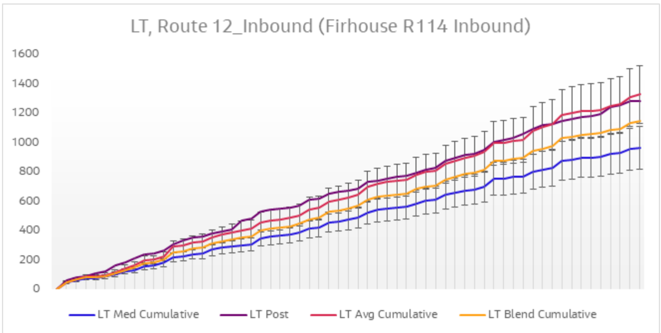
Diagram 6.18 Journey Time Validation Plot - Route 12 Inbound LT
