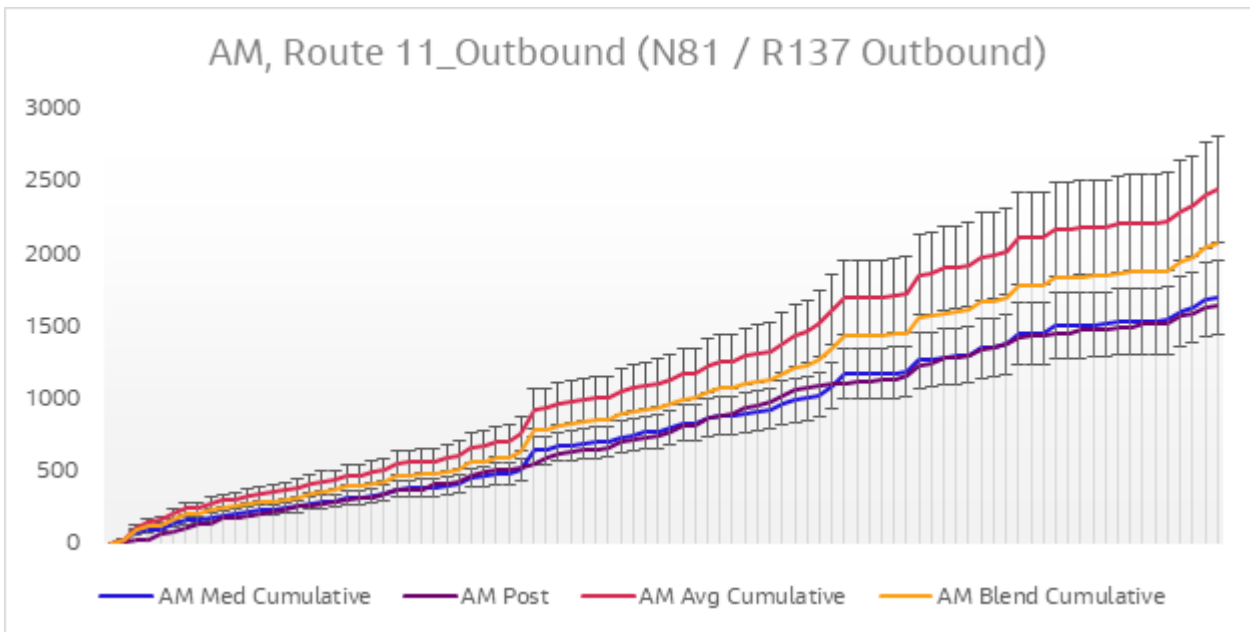
Diagram 6.13 Journey Time Validation Plot - Route 11 Outbound AM
