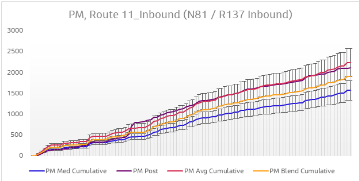
Diagram 6.24 Journey Time Validation Plot - Route 11 Inbound PM
