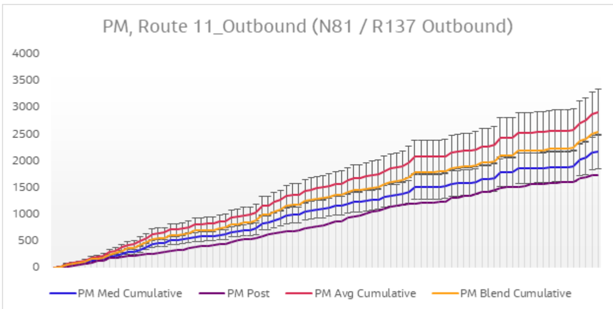
Diagram 6.25 Journey Time Validation Plot - Route 11 Outbound PM
