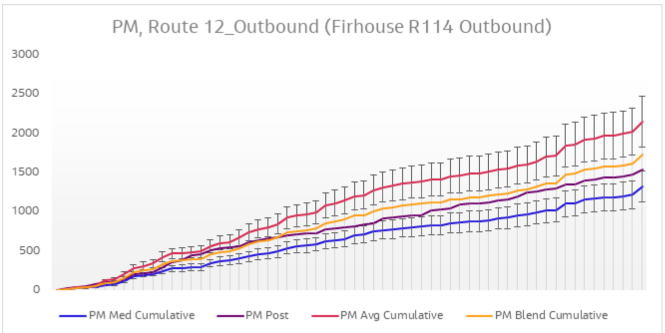
Diagram 6.27 Journey Time Validation Plot - Route 12 Outbound PM
