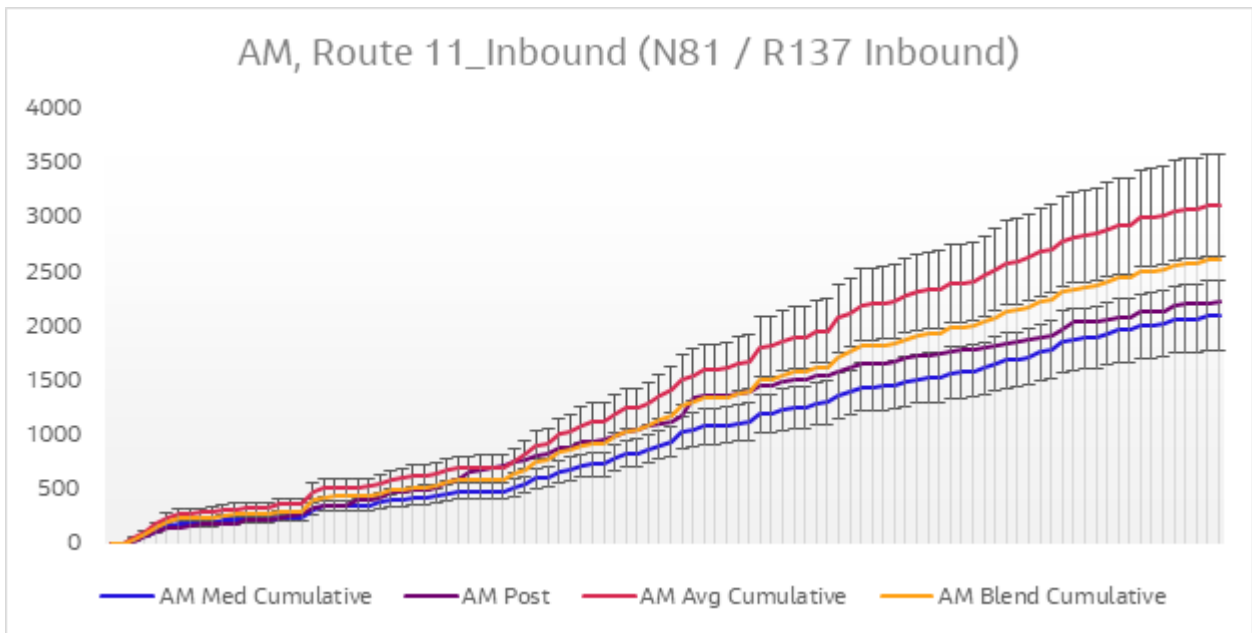
Diagram 6.12 Journey Time Validation Plot – Route 11 Inbound AM
