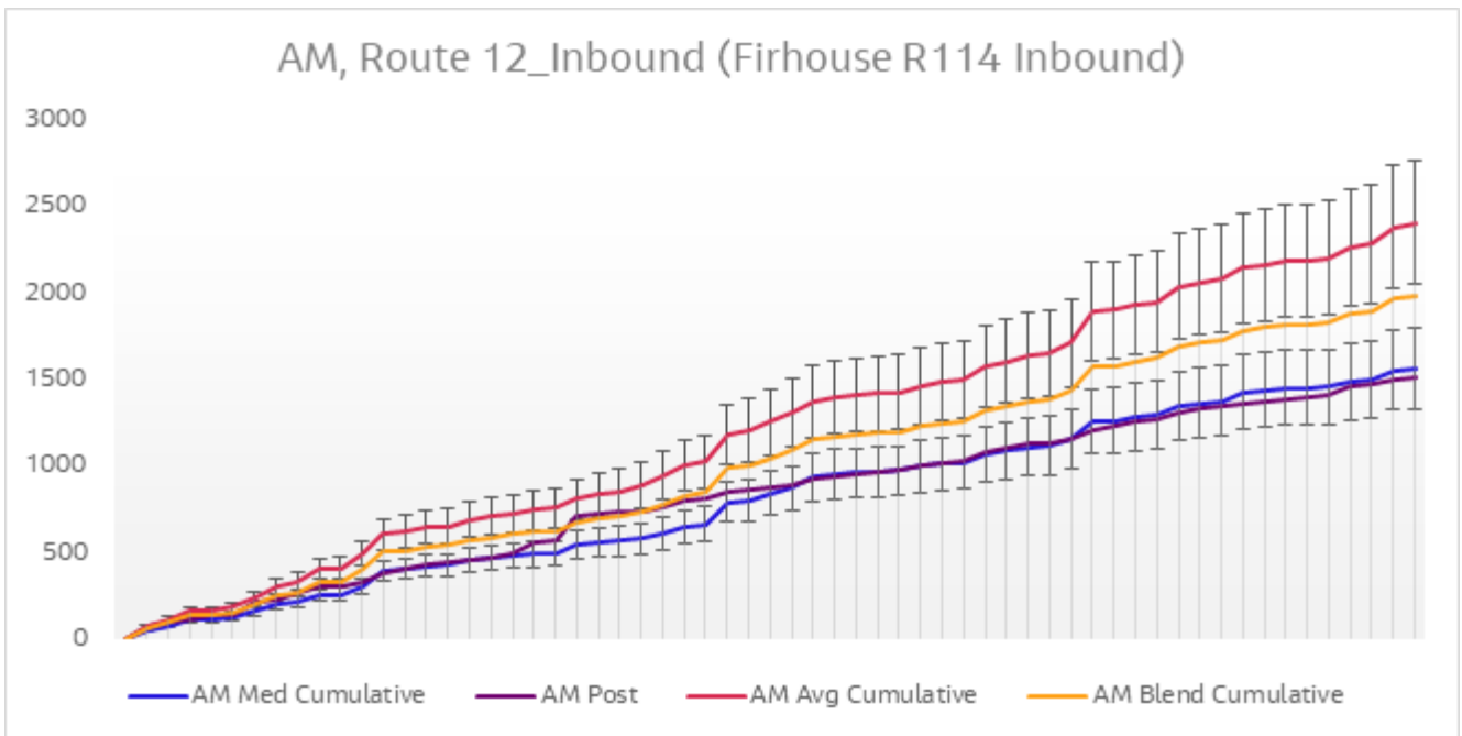
Diagram 6.14 Journey Time Validation Plot - Route 12 Inbound AM
