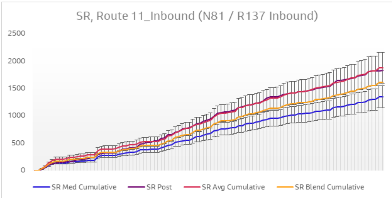
Diagram 6.20 Journey Time Validation Plot - Route 11 Inbound SR
