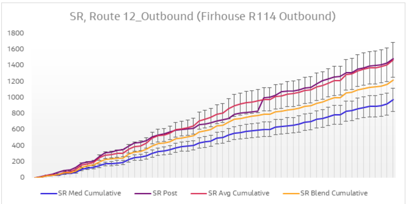
Diagram 6.23 Journey Time Validation Plot - Route 12 Outbound SR
