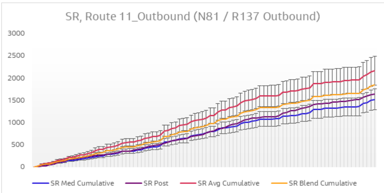
Diagram 6.21 Journey Time Validation Plot - Route 11 Outbound SR
