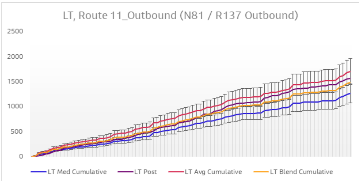
Diagram 6.17 Journey Time Validation Plot - Route 11 Outbound LT
