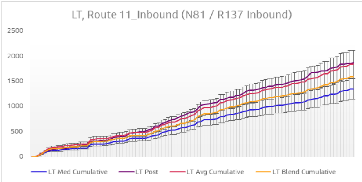
Diagram 6.16 Journey Time Validation Plot - Route 11 Inbound LT
