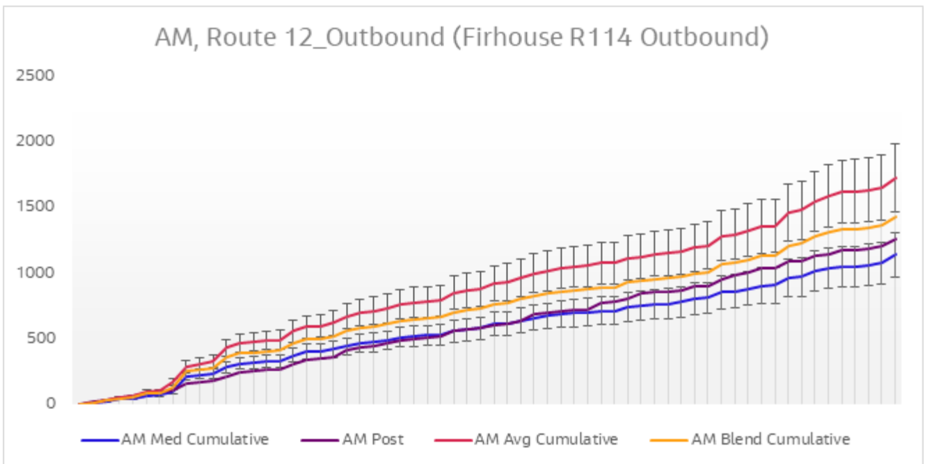
Diagram 6.15 Journey Time Validation Plot - Route 12 Outbound AM
