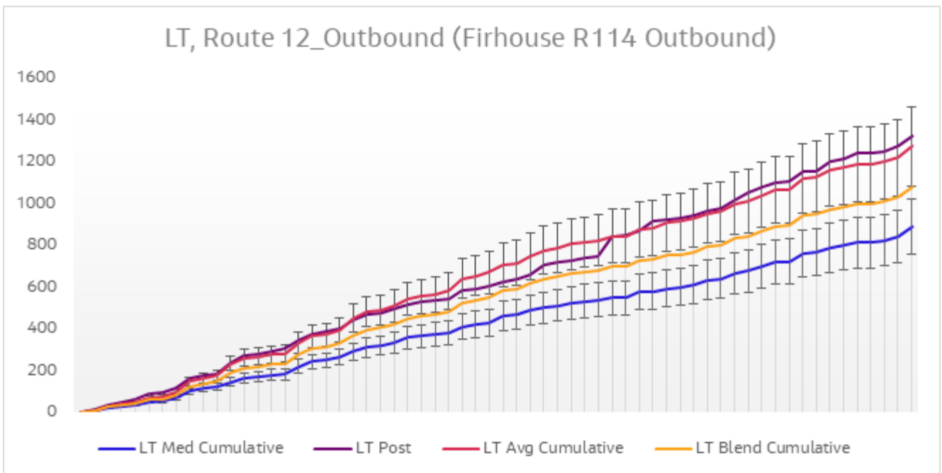
Diagram 6.19 Journey Time Validation Plot - Route 12 Outbound LT
